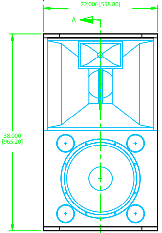
FRONT VIEW W/GRILL REMOVED
